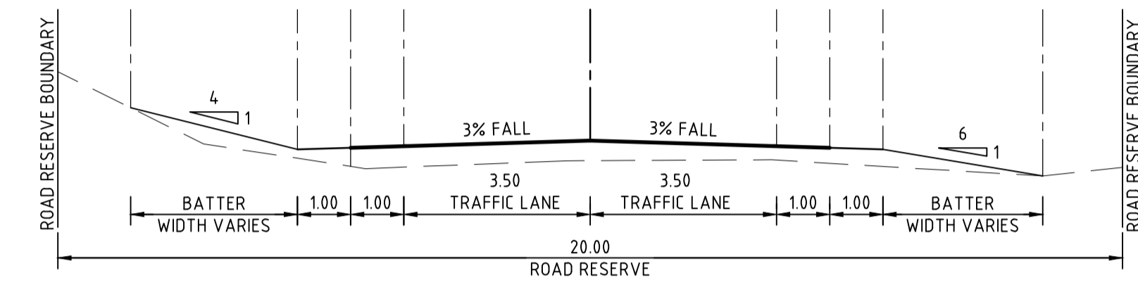
TYPICAL ROAD CROSS SECTION (NON BUILT UP AREAS) N.T.S.
