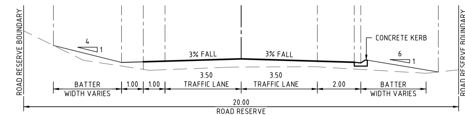
TYPICAL ROAD CROSS SECTION (WITH KERBING IN BUILT UP AREA) N.T.S.
